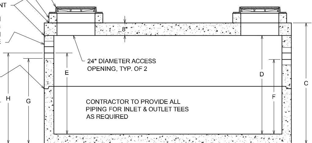
SECTION VIEW
