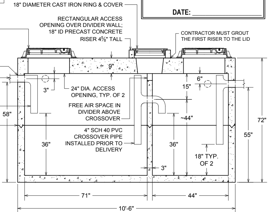
SECTION VIEW
