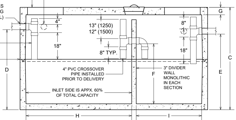
SECTION VIEW
