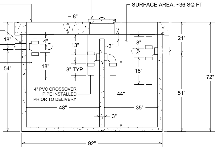
SECTION VIEW
