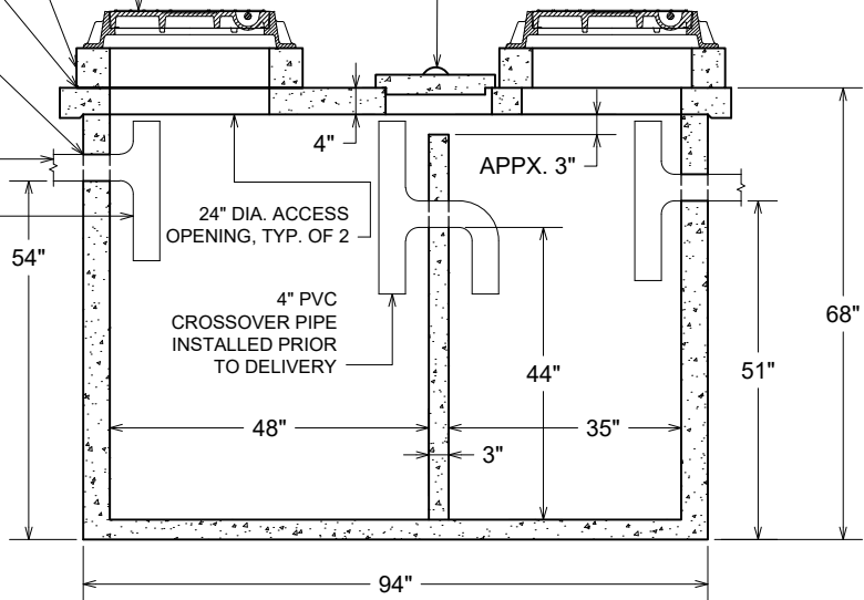
SECTION VIEW
