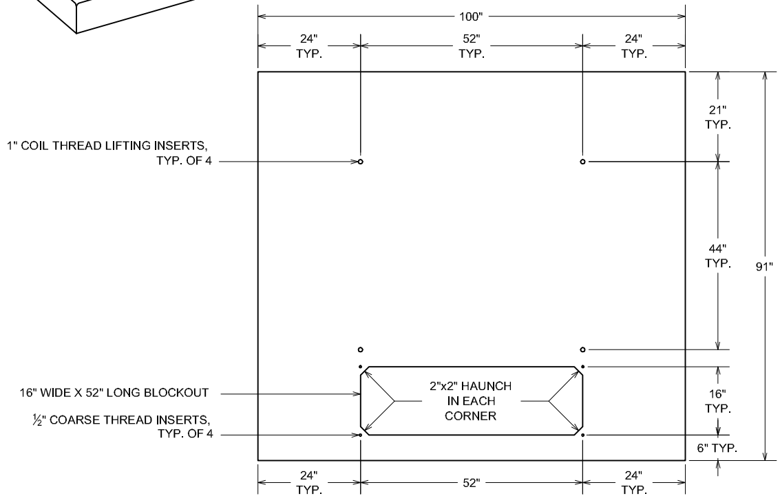
PLAN VIEW
