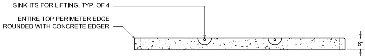
SECTION VIEW
